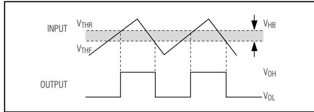
Figure 3. Hysteresis
